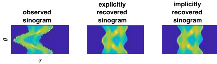
FIG. 11. (Left) Multiple CoR shifts introduce jitters in the measurement data. (Middle) the explicit approach provides a more clean and jitter-free sinogram. (Right) The implicit approach is also able to recover a clean and jitter-free sinogram.
