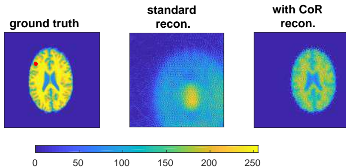
FIG. 15. (Left) Object as the standard MRI image with only one CoR shift denoted by the red dot. (Middle) Reconstruction from noise-free data without error recovery. (Right) Reconstruction with error recovery.
