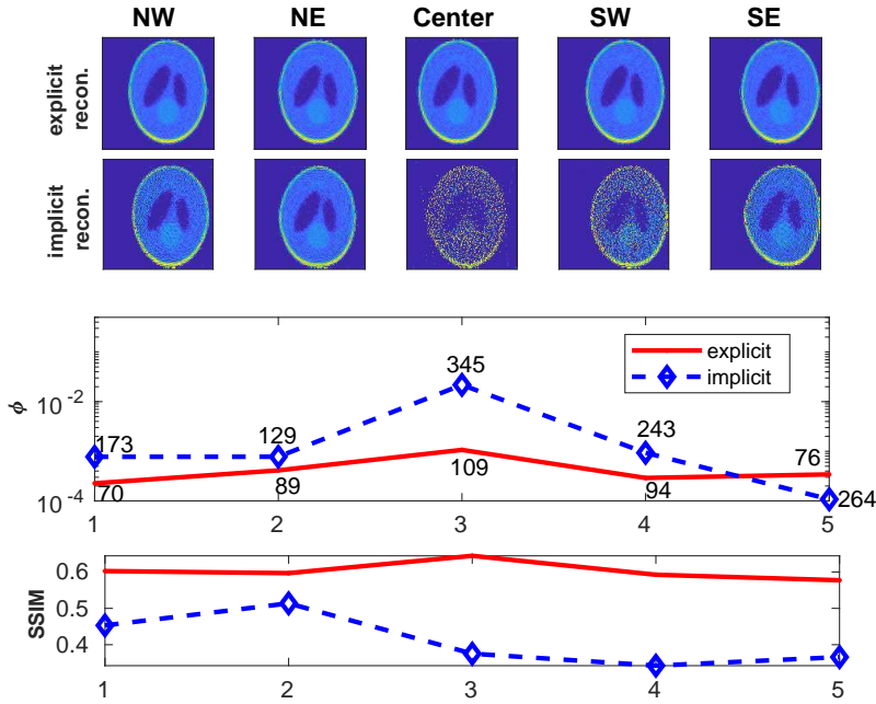
FIG. 9. Performance of the explicit and implicit approaches for recovering single CoR shift. Columns correspond to different initializations for CoR (x_g^*, y_g^*) . The top row shows the corresponding reconstructions from the explicit approach; the second row shows the corresponding reconstructions from the implicit approach; the third row shows the corresponding objective function values from the explicit and implicit approaches, respectively, where the number labeled on each case is the total number of iterations needed for convergence; the fourth row shows the reconstruction qualities measured
