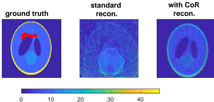
FIG. 12. (Left) Shepp-Logan phantom object with true CoRs connected by red dots. (Middle) Without error recovery, a direct reconstruction result is far away from the ground truth. (Right) Reconstruction result with error recovery, which is very close to ground truth.
