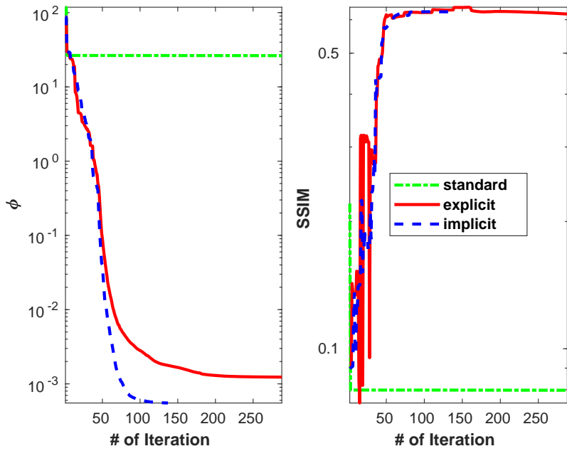
FIG. 14. Iterative performance of three approaches—standard tomographic reconstruction, explicit reconstruction, and implicit reconstruction—for multiple CoR-shift case. Left: progress of reducing objective value \phi . Right: progress of improving SSIM.
