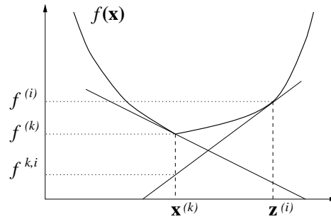
Figure 1: Shifted value f^{k,i} = f(\mathbf{z}^{(i)}) + g(\mathbf{z}^{(i)})^T(\mathbf{x}^{(k)} - \mathbf{z}^{(i)})
